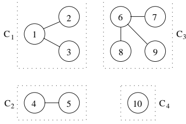
Fig. 1. A forest with 10 nodes and 4 clusters
