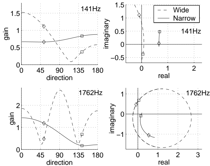
Figure 7: Directivity patterns (left) and their plot on complex planes (right)
