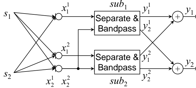
Figure 2: System structure
