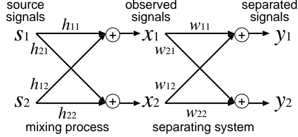
Figure 1: BSS model
