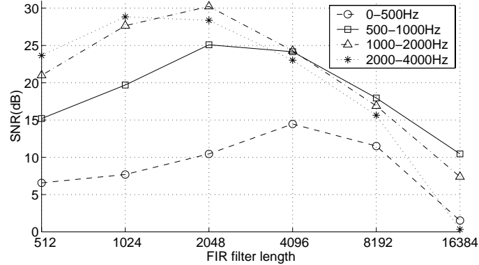
Figure 8: Effect of FIR filter length in frequency ranges
