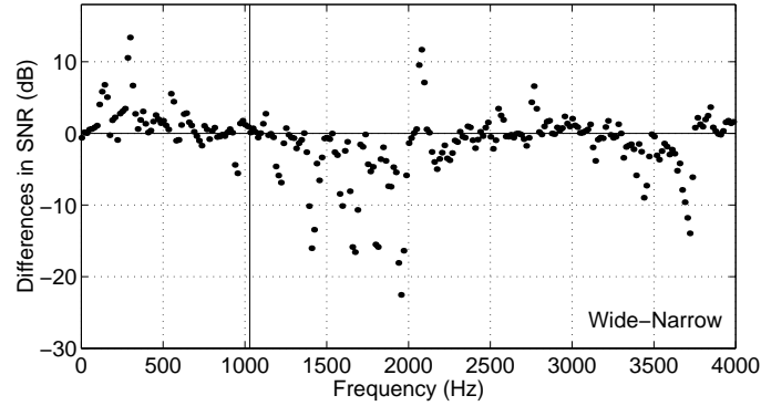
Figure 6: Differences in SNR at various frequencies
