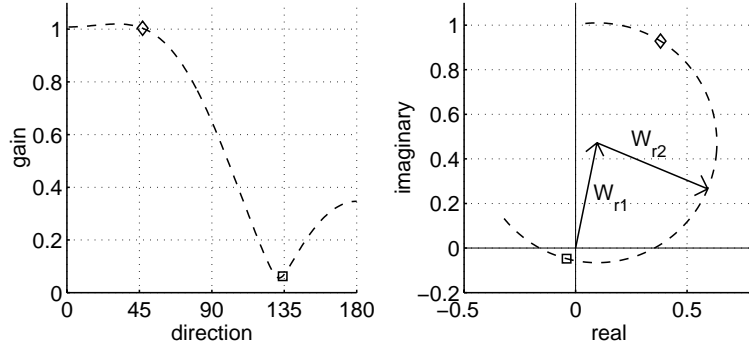
Figure 4: A directivity pattern (left) and its plot on a complex plane (right)
