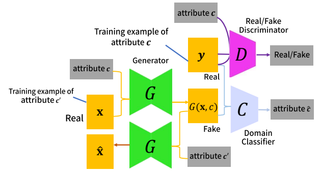
Fig. 3. Overview of StarGAN-VC training [13], [14].
