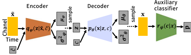
Fig. 2. Overview of ACVAE-VC training [15]. \tilde{x} and x denote acoustic feature sequences. \tilde{c} and c denote speaker information. z denote latent variable. q_\phi(z|\tilde{x}, \tilde{c}) output the mean \mu_\phi and variance \sigma_\phi^2 of the latent variable z following a normal distribution. p_\theta(x|z, c) output the mean \mu_\theta and variance \sigma_\theta^2 of the x that follows a normal distribution. r_\psi(c|x) output distribution p which speaker uttered the acoustic feature sequences x .
