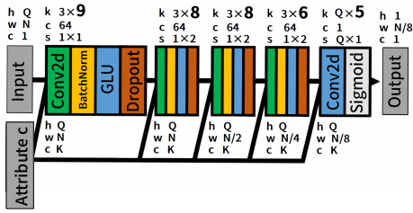
Domain Classifier
