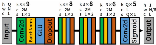
Domain Classifier
